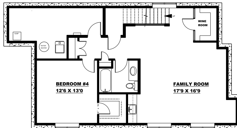
BASEMENT FLOOR PLAN 1127 SQ. FT 10'0 CONC. WALL
