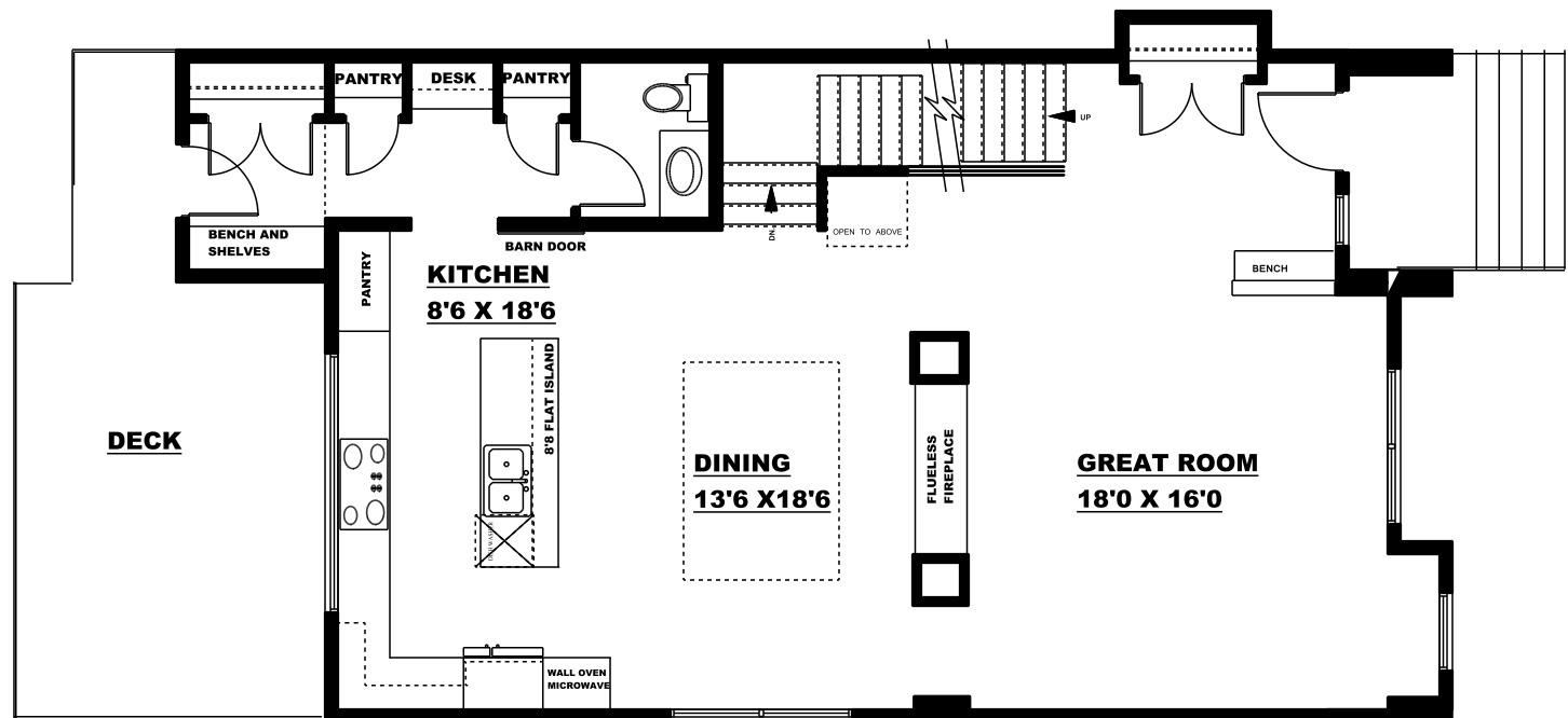
MAIN FLOOR PLAN 1136 SQ FT 10'0 CEILING
